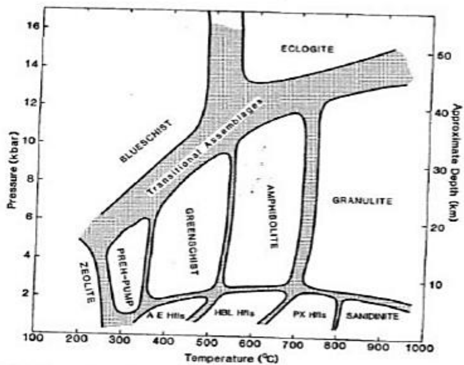
Fig. 2.8 Pressure-temperature diagram showing the fields of the various metamorphic facies. Details of the characteristic assemblages are given in Chapter 4 (Table 4.1). Abbreviations used are: Hfs = hornfels, AE = albite-epidote, HBL = hornblende, PX = pyroxene, PREH-PUMP = prehnite-pumpellyite.
